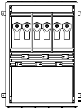
ABJB X3 (0-2) Cables entering from bottom only
